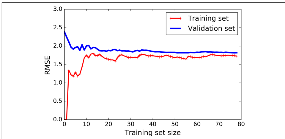
Figure 4-15. Learning curves
