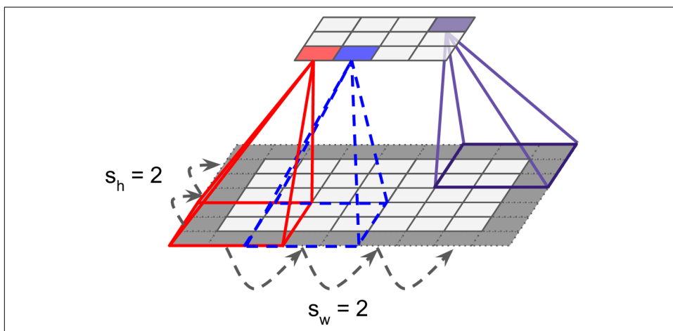
Figure 13-4. Reducing dimensionality using a stride of 2
