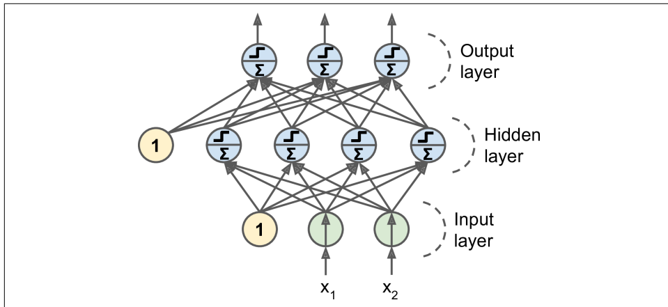
Figure 10-7. Multi-Layer Perceptron
