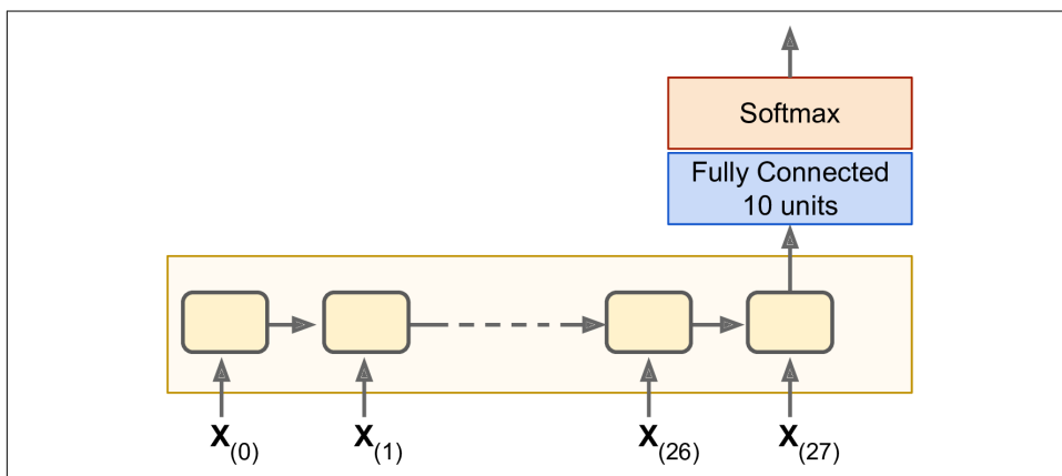
Figure 14-6. Sequence classifier
